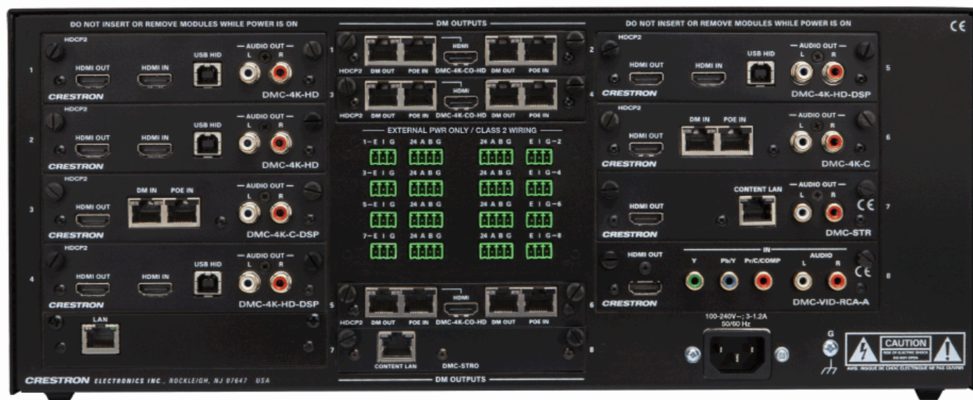
DM-MD8X8-RPS – Rear view with I/O cards installed
